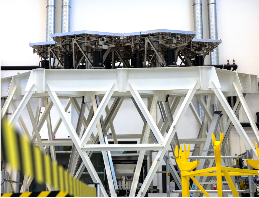
Above: Testing of ELT M1 segment supports at the ESO Headquarters.
