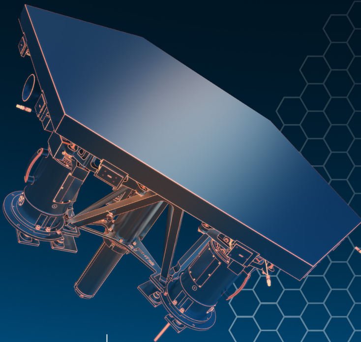
Artist's impression of one of the 798 segments of the ELT's primary mirror.
