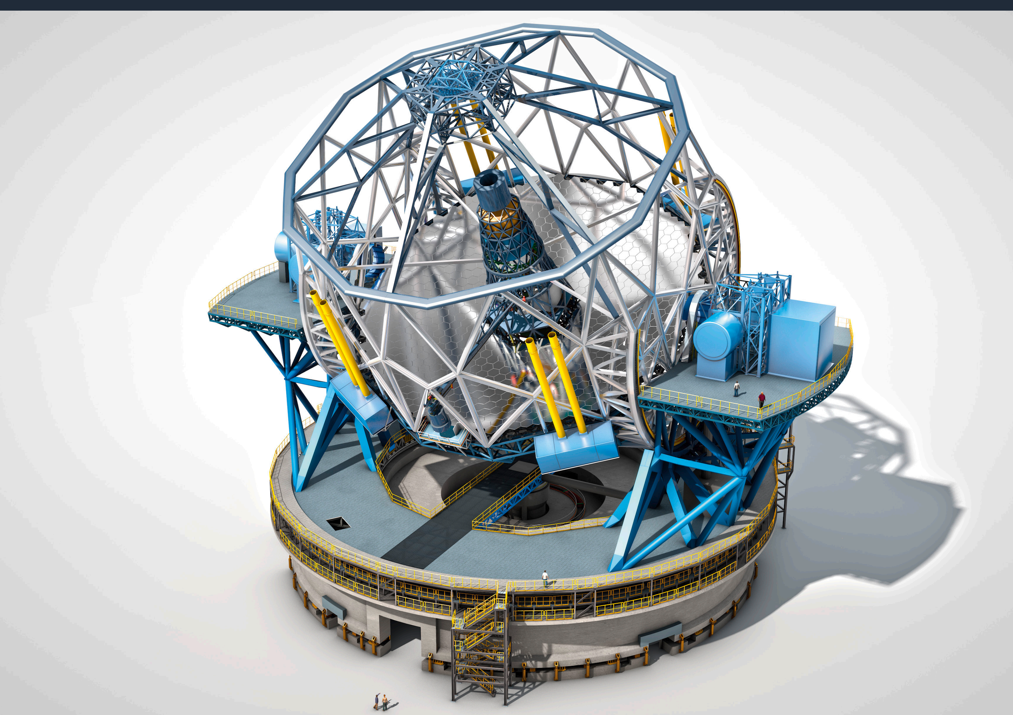
Artist's impression of the E-ELT design.
