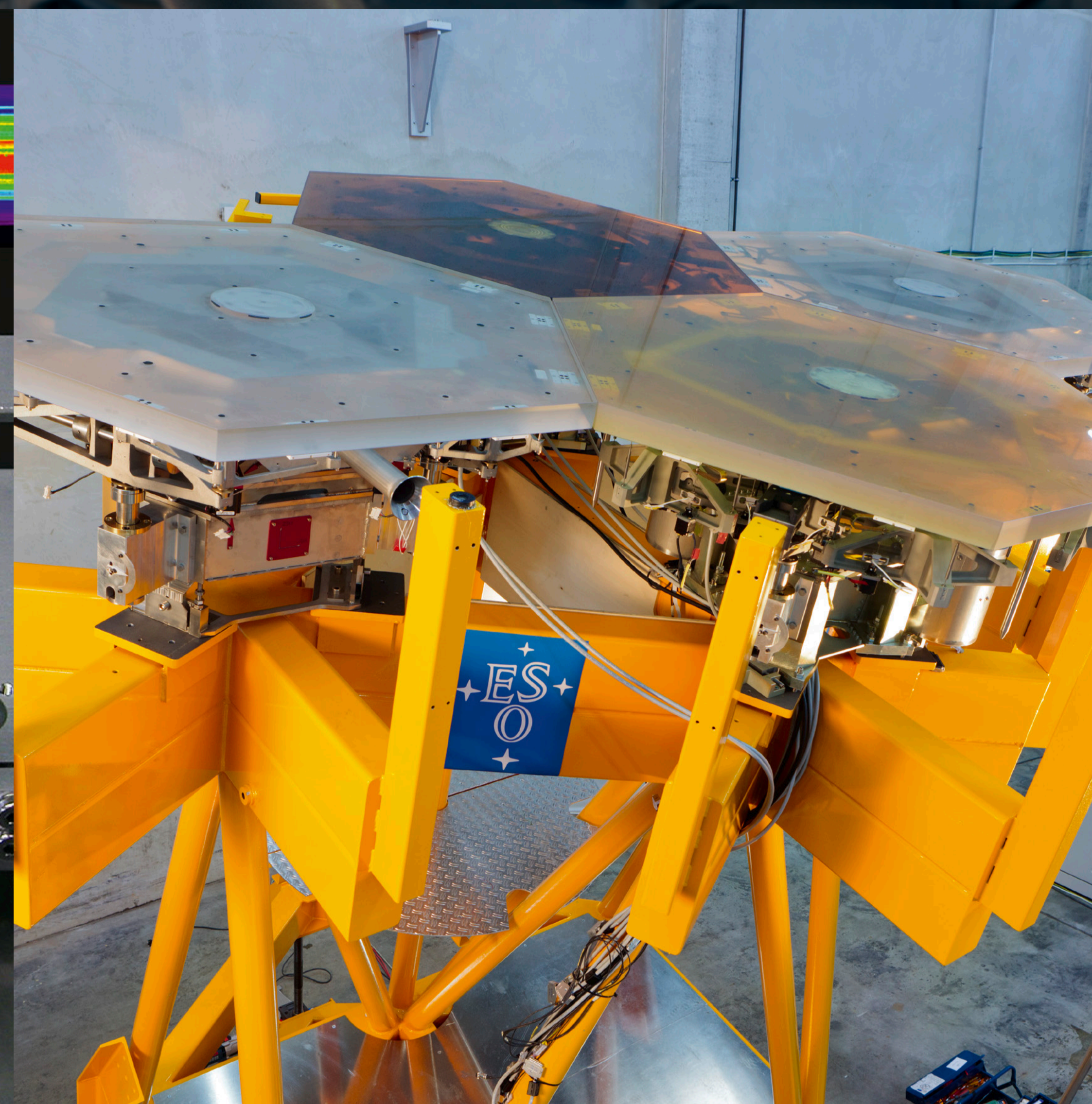
Experimental segments of the giant primary mirror of ESO-ELT undergoing testing. Credit: ESO/H. H. Heyer
