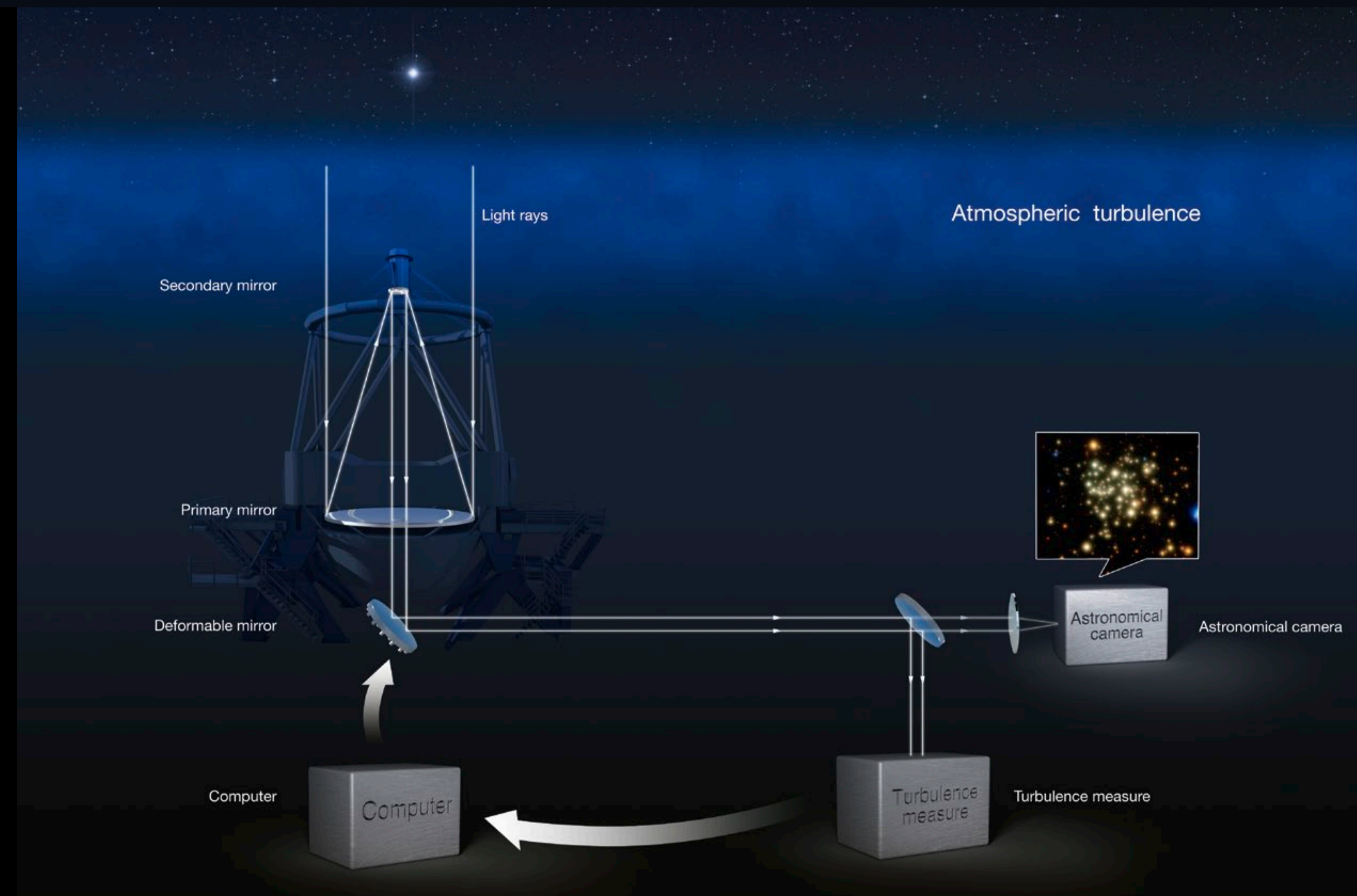
Illustrating the principle of adaptive optics.
