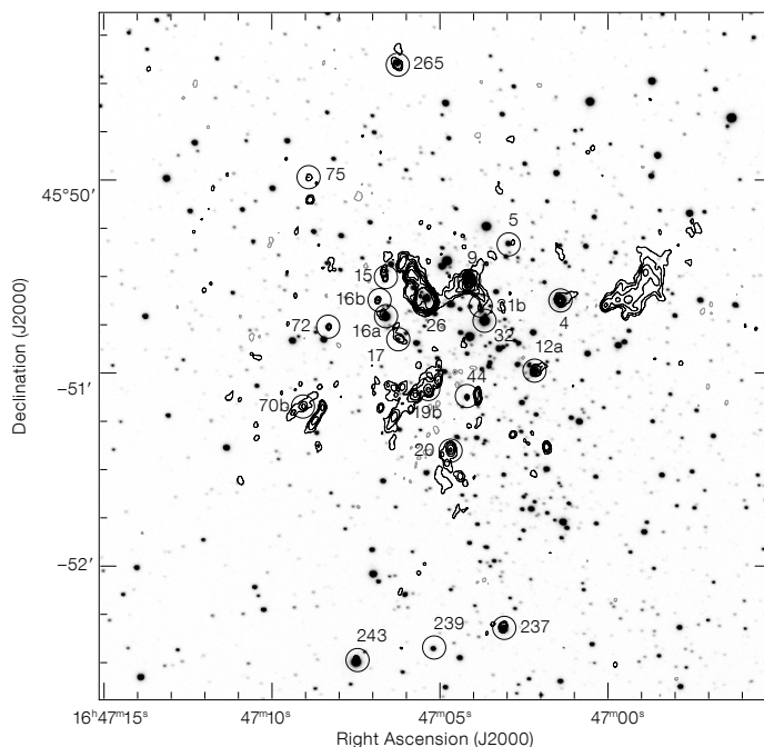
Figure 3. Overplot of radio observations (contours) on an optical image of Wd1. Note the emission associated with the cool hypergiants (Wd1-4, 12a, 16a, 32 & 265 — YHG; Wd1-20, 26 & 237 — RSG) indicative of significant ongoing mass loss.
