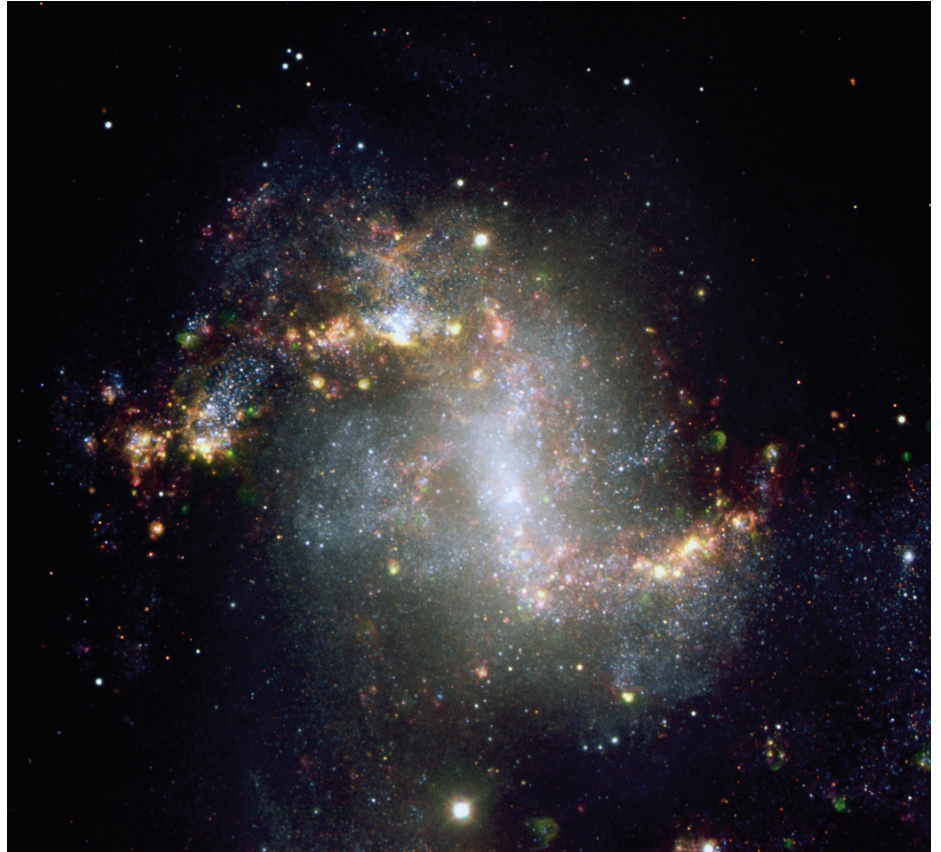
Figure 1. The central region of the vigorous starburst galaxy NGC 1313 is shown in this colour image from VLT FORS data (from Release eso0643). Note the numerous shells of ionised gas excited by young massive clusters similar to Wd1.
