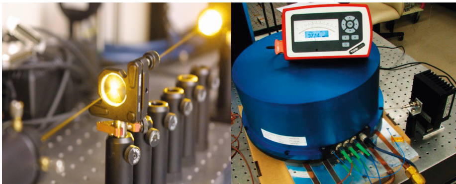
Figure 8. The optical tube assembly being developed by TNO Science & Industry. Together with the beam control and diagnostics system this assembly makes up the launch telescope system for the 4LGSF. Four similar units are mounted on the centrepiece of the UT to launch the four laser guide stars at 90 km altitude.
