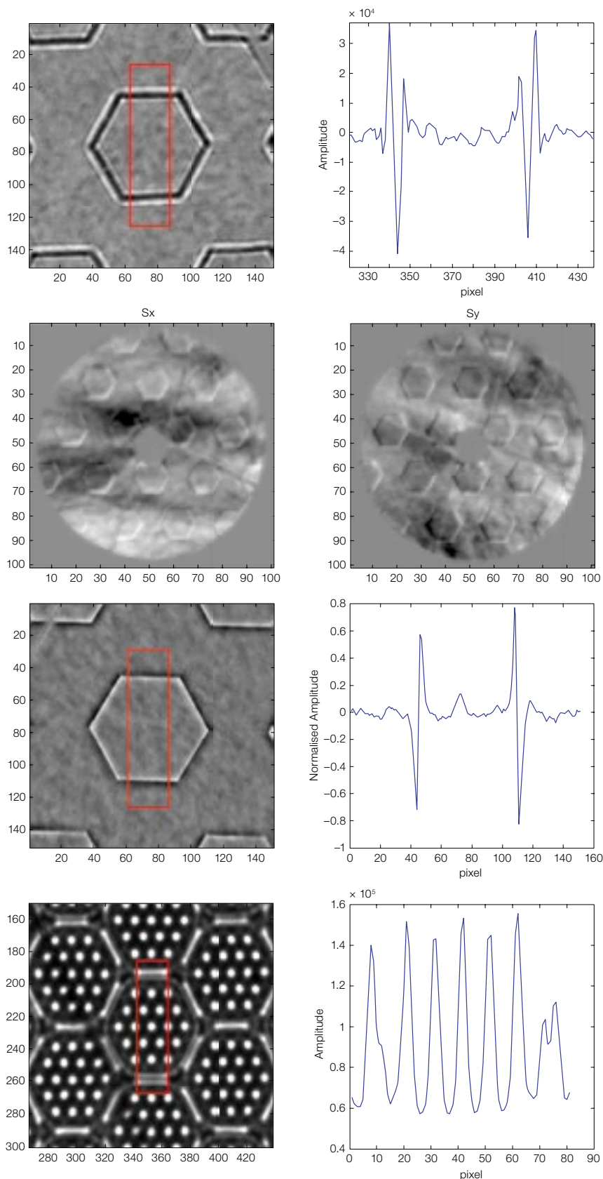
Figure 3. Typical images and signal cross-sections through active segments obtained with the four optical phasing sensors (DIPSI, PYPS, ZEUS and SHAPS, shown top to bottom) during on-sky observations with a wavefront piston step of 150 nm (except SHAPS with steps of 150 nm and 300 nm) and seeing conditions between 0.8" and 1.2". All image units are pixels.
