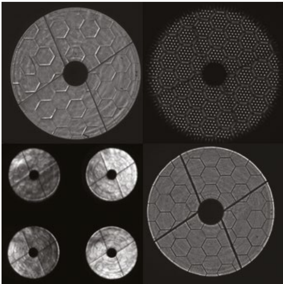
Figure 6. Raw first light signals of the "segmented" primary mirror of the VLT obtained by the four optical phasing sensors. Top row: ZEUS, SHAPS; bottom row: PYPS, DIPSII.
