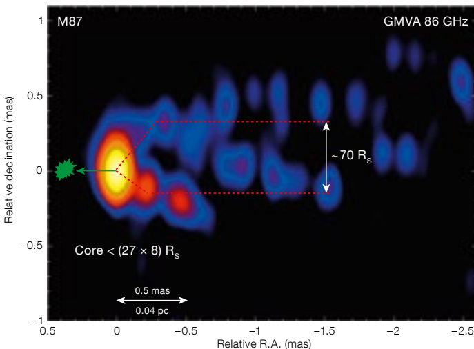
Figure 3. Left: 86 GHz VLBI image of the jet in M87 (from Krichbaum et al., 2007). The jet extends down to some tens of Schwarzschild radii (Hada et al., 2011). Right: A 43 GHz VLBA image from Walker et al. (2008), clearly revealing the limb-brightened structure also seen at 86 GHz.
