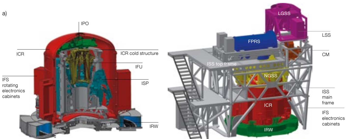
Figure 2. a) Cutaway CAD model of the HARMONI cryostat (ICR), situated on the instrument rotator and cable wrap (IRW). The view shows the main opto-mechanical components of the integral field spectrograph (IFS), namely the IFS pre-optics (IPO), the integral field unit (IFU), and the spectrographs (ISP). b) overall CAD assembly of HARMONI, with the various systems comprising the instrument coloured differently. The LSS is the LGSS Support Structure. Other acronyms are explained in the text.
