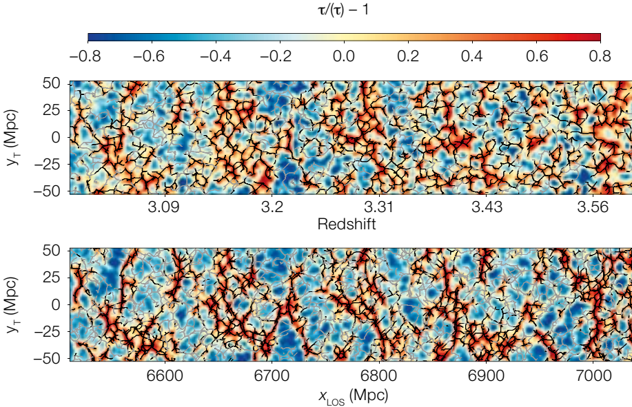
Figure 3. Simulations of MOSAIC performance when observing simultaneously the ISM absorption lines in the spectra of numerous R_{AB} \leq 25.5 Lyman break galaxies enabling a vast area (100 Mpc in diameter) of the sky plane to be sampled. This allows the study of 10-Mpc-thick longitudinal slices lying from redshift 3 to 3.6, of the simulated (top, signal-to-noise ratio = 4) and original (bottom) optical depth contrast field ( \tau/\langle\tau\rangle - 1 ), where \tau = -\log F and F is transmitted flux ( \tau is taken as a proxy for the HI density). The y -axis is the projected transverse dimension ( y_T ). Filaments extracted are over-plotted in grey and black. The black lines correspond to the 50% densest filaments. As noise in the spectra increases, the reconstruction shows lower contrast, and filaments are more randomly located (from Japelj et al., 2019).
