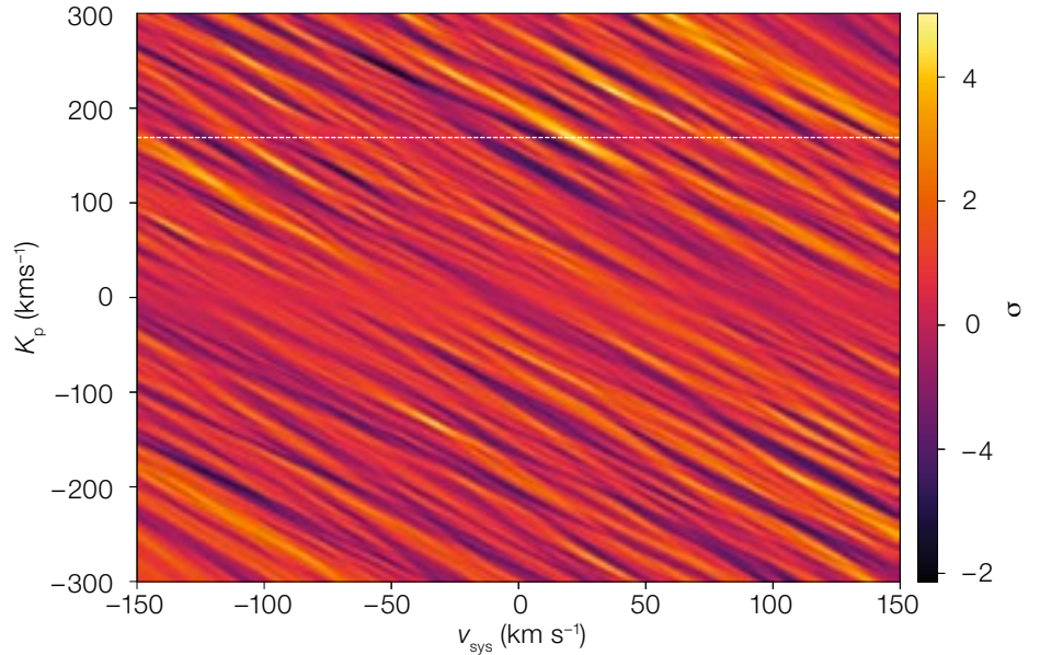
Figure 8. K_p - v_{sys} map of the summed cross-correlation signal for a H 2 O template. The plot shows a tentative detection of water near the expected K_p and v_{sys} at > 4\sigma ; however, refinements of the model templates are continuing in order to confirm the signal.
