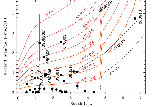
Fig. 3. The effect of the combination of various values of intrinsic extinction A_V (lines with labels) and redshift, producing an effective dimming in the R band as given on the y -axis. The solid lines have been computed assuming a dust extinction curve as described in Reichart (1999) but with no 2175 Å bump and an opacity due to intergalactic hydrogen approximated by \tau(\text{HI}) = 2.6 \times (1+z)^{3.3} for 700 \text{ nm}/(1+z) \leq 121.6 \text{ nm} (Valageas, Schaeffer & Silk 1999). Dots represent the GRBs of our sample for which we have an A_V measurement from the GROND SED. GRBs with effective R -band reduction of >0.5 mag are labeled; GRBs 080218B and 080915 lie above the corresponding labeled dashed lines which correspond to the pairs of (z, A_V) values described in the text. Moderate A_V at moderate redshifts can easily produce a dimming of 1–3 mag in the R band.
