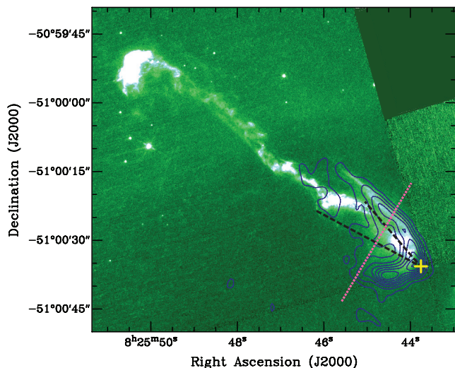
FIG. 6.— Comparison of blue CO lobe and optical image of HH 46/47 jet. The HST image was taken with the [SII] (F673N) filter in 2008 by Hartigan et al. (2011). Contours show the emission integrated over the velocity range from -6.8 to -3.2 \text{ km s}^{-1} . This velocity range was chosen to avoid contamination from cloud emission and B0. The lowest contour and subsequent contour steps are 0.15 and 0.2 \text{Jy beam}^{-1} \text{ km s}^{-1} , respectively. The yellow cross shows the position of HH 47 IRS. The two black dash lines connect the position of the source to outermost positions of the wiggling jet, with respect to the outflow axis. The dotted pink line perpendicular to the outflow cavity shows the position of the p-v cut shown in Figure 10a.
