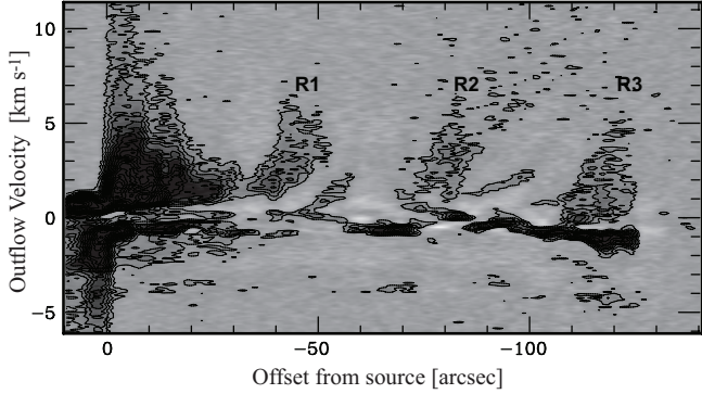
FIG. 9.— Position-velocity diagram along the axis of the red lobe. The figure was constructed using a map with velocity resolution of 0.08 \text{ km s}^{-1} , with a position angle of 60^\circ , and summing the emission over a 7.5'' -wide cut. The lowest contour and subsequent contour steps are 1 and 1.5 \text{ Jy beam}^{-1} , respectively. The positions of the redshifted outflow clumps along the outflow axis are shown.
