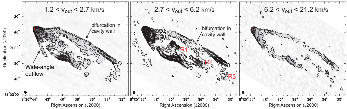
FIG. 7.— Velocity range-integrated intensity maps of the CO redshifted emission. The velocity interval of integration is given at the top of each panel. In the left, middle and right panels the lowest contour and contour steps are 0.2, 0.105, and 0.2 Jy beam -1 km s -1 , respectively. The synthesized beam is shown on the lower left corner of each panel. The red cross shows the position of HH 47 IRS.
