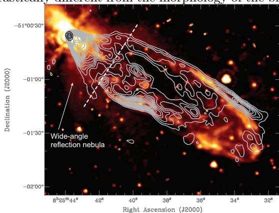
FIG. 8.— Comparison of red CO lobe with Spitzer IRAC 2 (4.5 \mu m) image. The Spitzer data are from Noriega-Crespo et al. (2004) and have been reprocessed with a deconvolution algorithm to reach an angular resolution of \sim 0.6 - 0.8'' , with 60 iterations (see Noriega-Crespo & Raga 2012 for details). White contours show the integrated intensity of the CO redshifted lobe (the same as shown in Figure 1). Black contours show the 3 mm continuum emission around HH 47 IRS. The lowest contour and subsequent contour steps are 2 mJy beam -1 . The white dash line shows the position of the p - v cut shown in Figure 10b.
