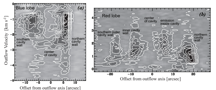
FIG. 10.— Position-velocity diagrams perpendicular to the outflow axis for the blue (left panel) and red (right panel) lobes. In both p-v diagrams the offsets are given with respect to the position of the outflow axis in the cut. The location of the p-v cuts for the blue and red lobes are shown in Figures 6 and 8, respectively. In the left panel the lowest contour and the subsequent contour steps are 0.2 and 0.15 \text{ Jy beam}^{-1} , respectively. In the right panel the lowest contour and the subsequent contour steps are 0.07 and 0.16 \text{ Jy beam}^{-1} , respectively.
