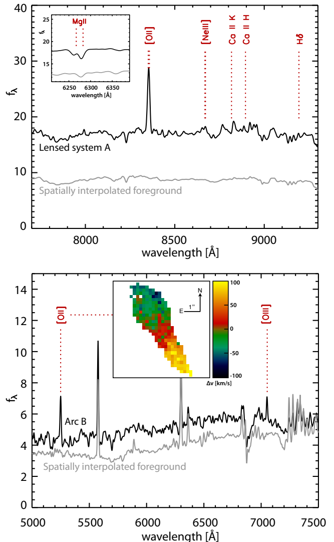
Figure 2. Observed spectra at the locations of background galaxies A (top) and B (bottom). In both cases, the grey line shows the spectrum of nearby emission from the foreground cluster, spatially interpolated to the position of the background galaxy. The coloured insert shows galaxy B’s 2D velocity field in a 6'' \times 6'' region, for all IFU pixels where [OII] emission is detected at signal to noise > 4 . It indicates a rotationally supported disc.
