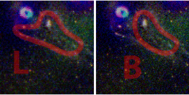
Figure B1. Two alternative configurations of lensed image associations near cluster galaxy N.4. There is a surprising high density of point sources, so it is not obvious which sources correspond to which lensed images. Configuration L is a small perturbation of the fiducial model in the main paper. Configuration B is based upon LENTOOL’s best-fit mass model if no identifications are initially made in this region. However, it is at odds with narrow-band imaging of the source, created from line emission in our VLT IFU data (see figure 3).
