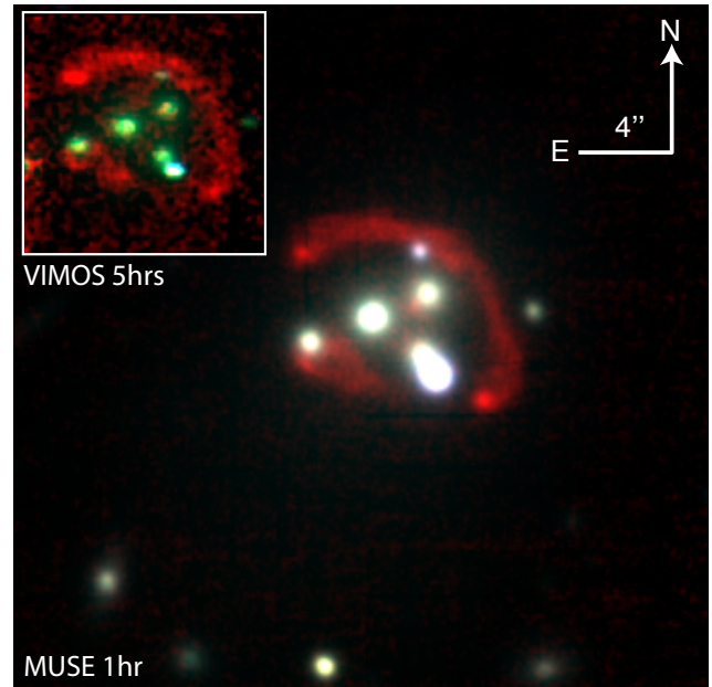
Figure A1. False-colour images of the cluster core, manufactured from the IFU 3D data cubes from VLT/VIMOS and VLT/MUSE . Red, green and blue channels in both images respectively correspond to a narrow-band [OII] image (created as described in section 3.2), Johnson I band and Johnson V band.
