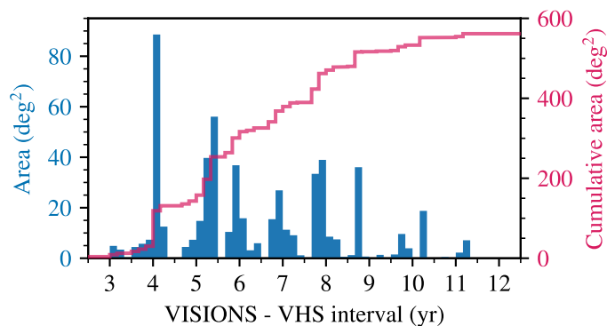
Fig. 6. Distribution of the maximum available time interval between VHS and VISIONS observations, constructed from the healpix grid in Fig. 5. The blue histogram shows the captured area as a function of the available time difference between the surveys. The red line displays the same statistic in cumulative form. As a consequence of the broad, multimodal range of available time baselines, the accuracy of derived proper motions will vary accordingly.
