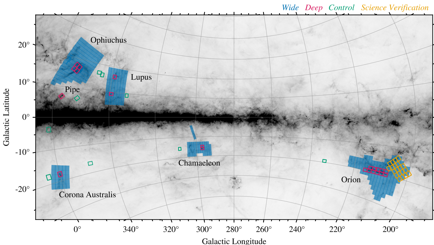
Fig. 3. Star-forming regions observed in the VISIONS survey plotted on top of Planck data at 857 GHz. The individual colors of the marked regions portray the subsurveys of the program. The filled blue tiles represent the coverage of the wide program, whereas the red and green rectangles indicate the on-sky locations of data collected as part of the deep and control observations, respectively. Science verification data, collected in the region of the Orion star forming complex, is depicted in orange.
