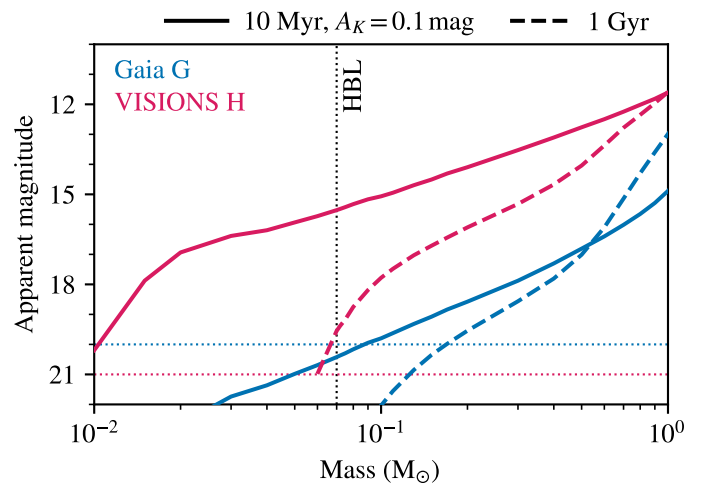
Fig. 8. Apparent magnitudes in the Gaia G (blue) and VISIONS H (red) passbands as a function of mass for objects at a distance of 400 pc. Solid lines represent a case of young stars with an age of 10 Myr located in a region with A_K = 0.1 mag foreground extinction. The dashed lines represent field stars at an age of 1 Gyr without any foreground extinction. The dotted vertical and horizontal lines mark the hydrogen burning limit (HBL) and the surveys’ sensitivity limits, respectively.
